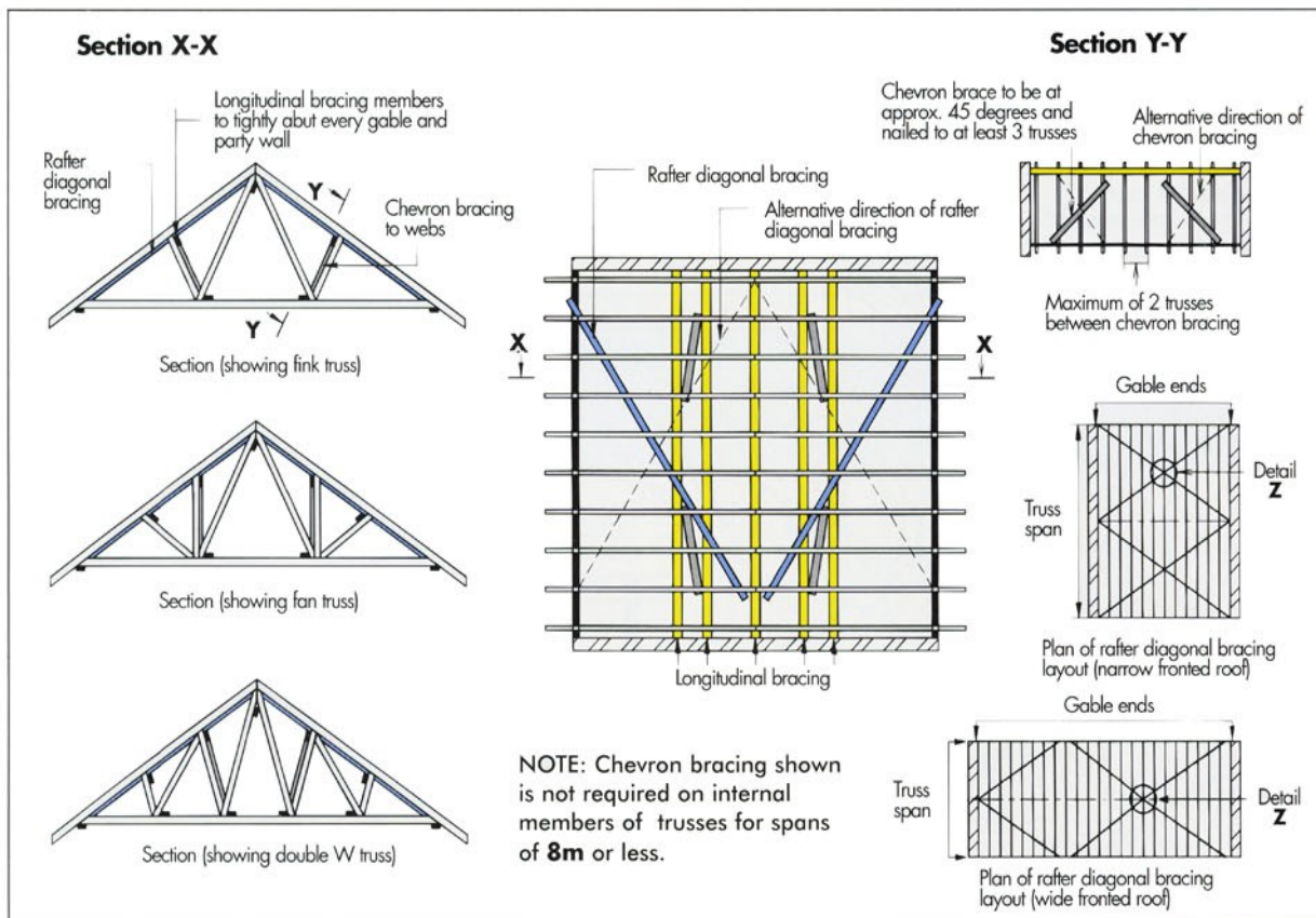
Diagram 2. Standard bracing for rafter and web members of duo-pitch trussed rafters.
