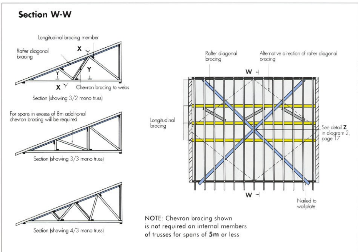
Diagram 1. Standard bracing for rafter and web members of mono-pitch trussed rafters.
